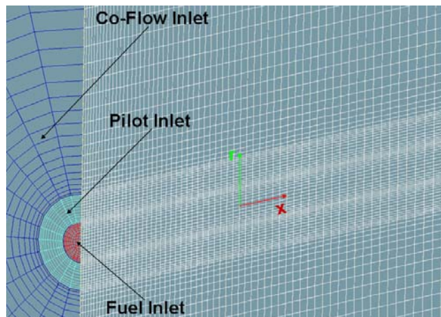
Figure 6.14: Computational mesh and inlet boundary conditions
