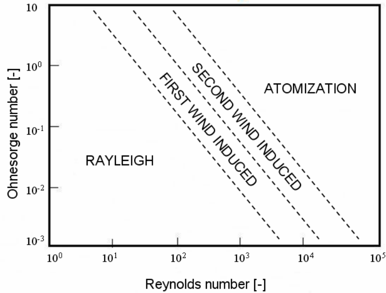
Figure 2.6: Liquid jet disintegration regimes
