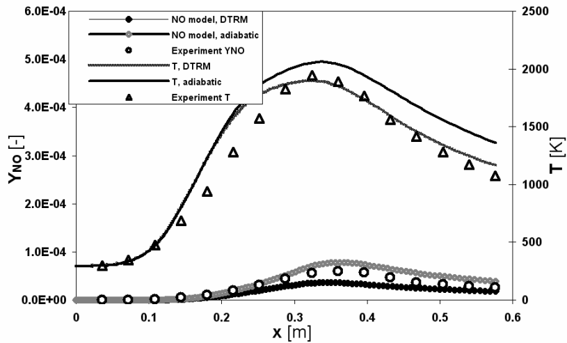
Figure 6.18: Axial profiles of mean temperature and mean NO mass fraction
