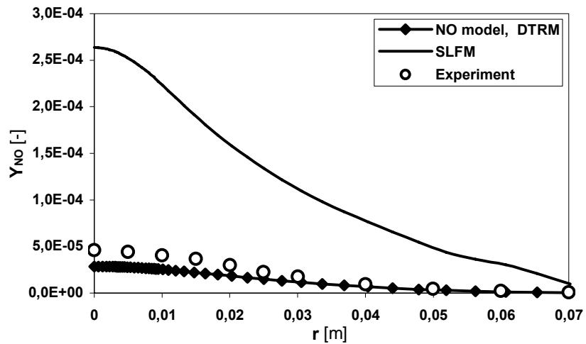
Figure 6.22: Radial profiles of mean NO mass fraction at axial distance x/d=60
