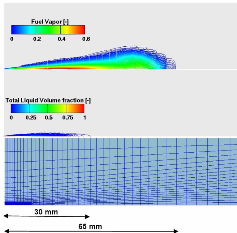
Figure 6.8: Total liquid volume fraction and vapor mass fraction 2 ms after start of injection
