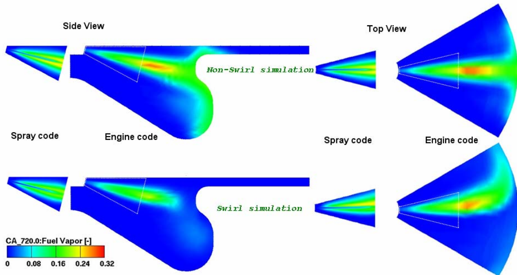
Figure 6.38: Fuel vapor of the spray and engine code at 720 deg CA
