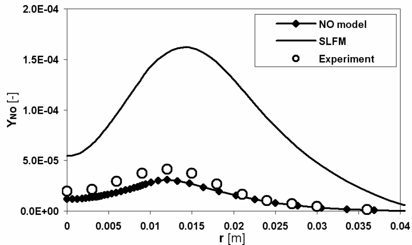
Figure 6.20: Radial profiles of mean NO mass fraction at axial distance x/d=30
