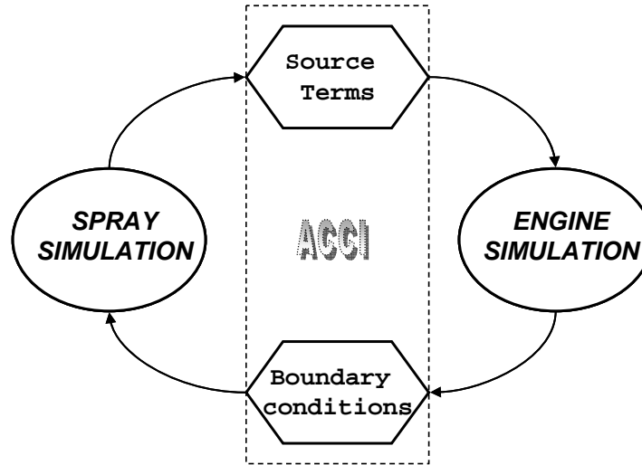
Figure 6.27: Data exchange in coupled simulations
