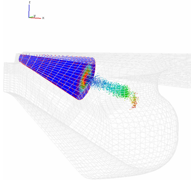
Figure 6.29: DDM parcels produced in the engine domain
