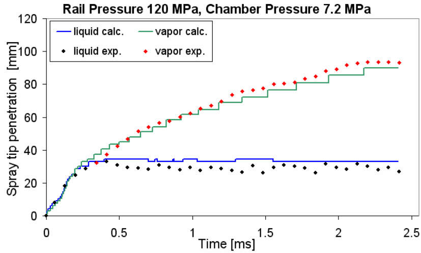
Figure 6.10: Comparison of the calculated and measured liquid and vapor penetration at 120 MPa rail pressure and 7.2 MPa chamber pressure
