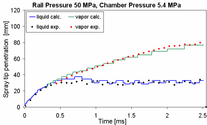
Figure 6.11: Comparison of the calculated and measured liquid and vapor penetration at 50 MPa rail pressure and 5.4 MPa chamber pressure
