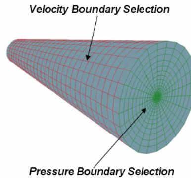
Figure 6.34: Spray mesh and boundary conditions used for calculation
