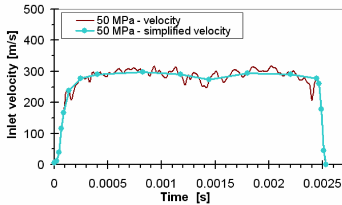
Figure 6.4: Inlet velocity profiles at 50 MPa rail pressure
