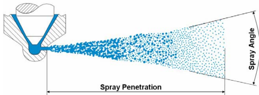
Figure 2.4: Schematic illustration of spray characteristics
