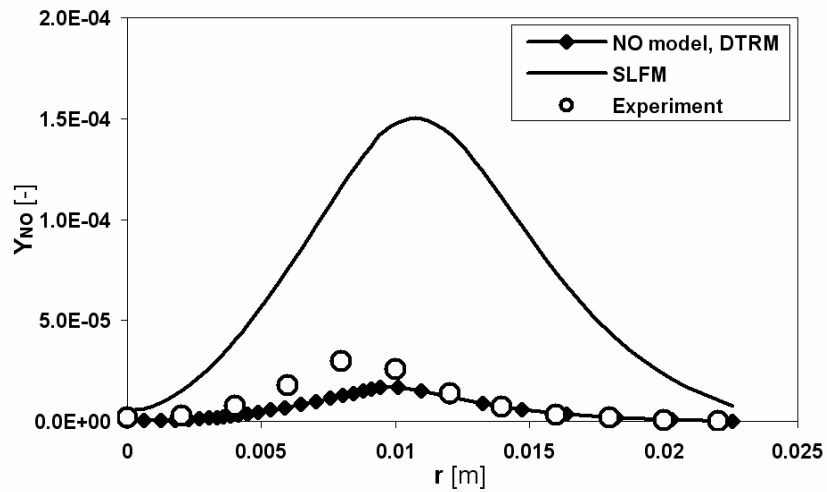
Figure 6.19: Radial profiles of mean NO mass fraction at axial distance x/d=15
