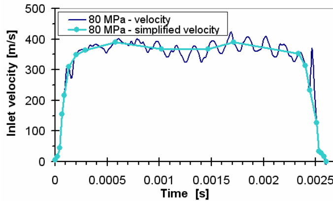
Figure 6.5: Inlet velocity profiles at 80 MPa rail pressure
