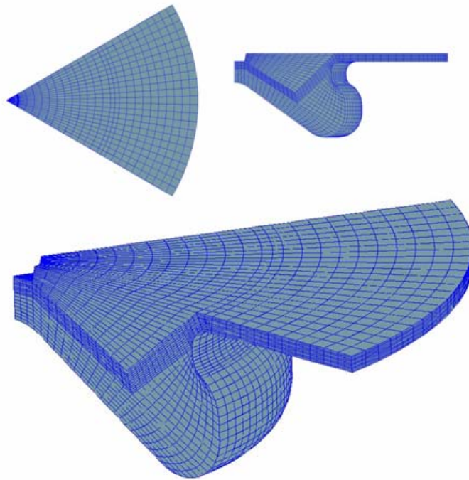
Figure 6.31: Engine mesh at TDC
