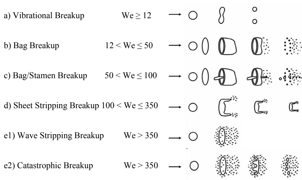
Figure 2.7: Droplet break-up mechanism by [59][60]
