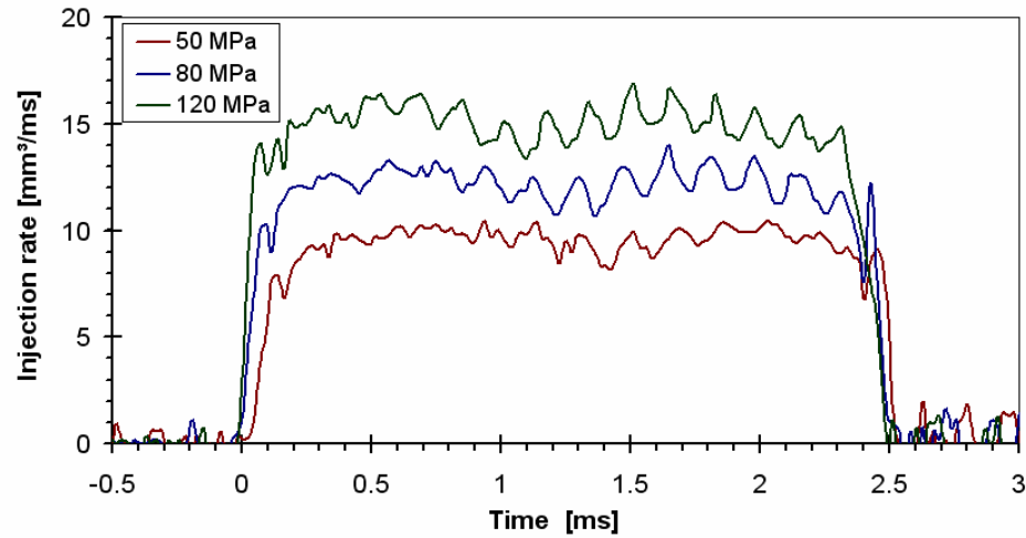
Figure 6.1: Injection rates for different injection pressures
