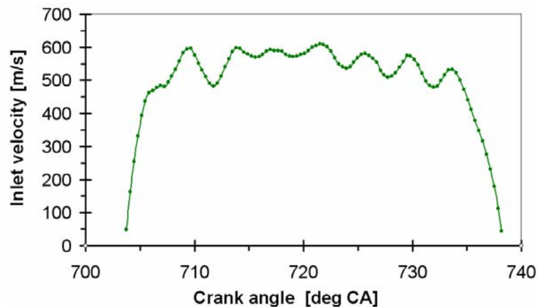
Figure 6.33: Injection velocity used for spray simulation
