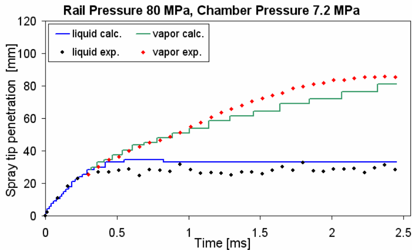
Figure 6.9: Comparison of the calculated and measured liquid and vapor penetration at 80 MPa rail pressure and 7.2 MPa chamber pressure
