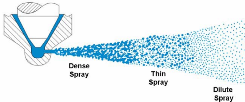
Figure 2.3: Schematic illustration of spray regimes
