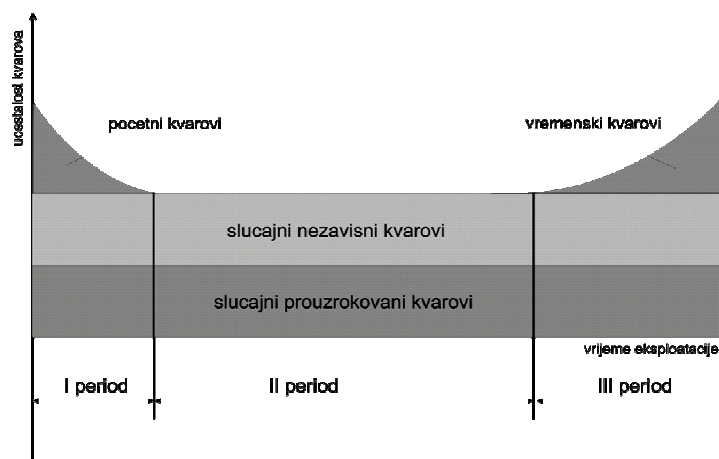
Slika 3.5 Krivulja kade ( Bathtub curve )
