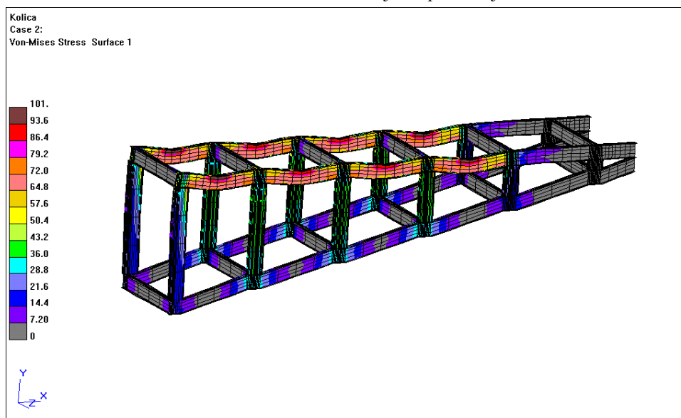
Fig. 10 Towing wagon 3D plate element model deformations and von Mises stresses
