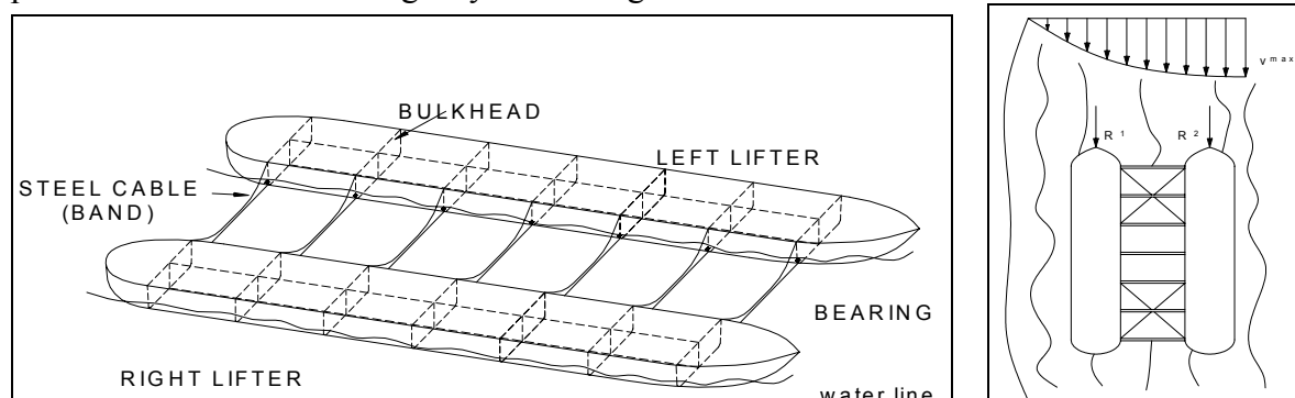
Fig. 1 Docking arrangement with two laid-up tankers floating in river current
