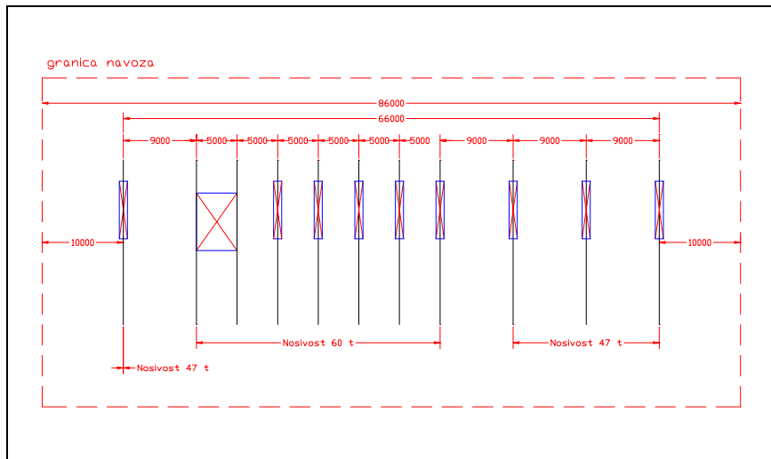
Fig. 7 Disposition of the groundways and towing wagons
