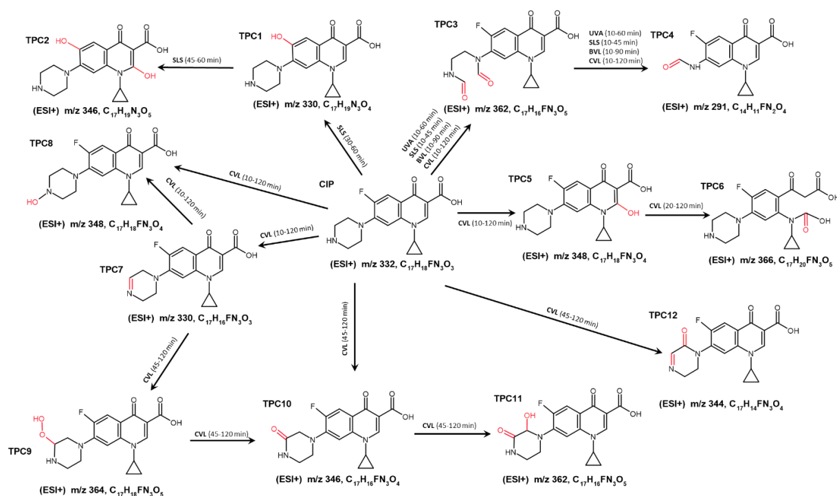
Figure 59. Ciprofloxacin pathways degradation by N/TiO 2 /rGO@Al 2 O 3 foam under UVA light (UVA), solar light simulator (SLS), blue visible light (BVL), and cold visible light (CVL).
