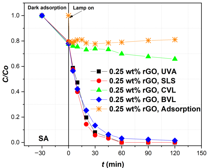
Figure 43. Adsorption and photocatalytic degradation of acid (SA) by N/TiO 2 /rGO with 0.25 wt. % of rGO material under UVA light, solar light simulator (SLS), cold visible light (CVL), and blue visible light (BVL).
