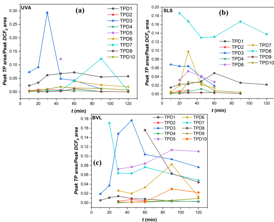
Figure 60. Transformation byproducts profile generated during the photocatalytic degradation of diclofenac (DCF) by N/TiO 2 /rGO@Al 2 O 3 foam under (a) UVA light, (b) solar light simulator (SLS), and (c) blue visible light (BVL).
