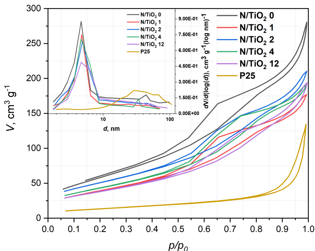
Figure 17. Adsorption-desorption isotherm, and pore size distribution of N/TiO 2 materials at different N/Ti molar ratios.
