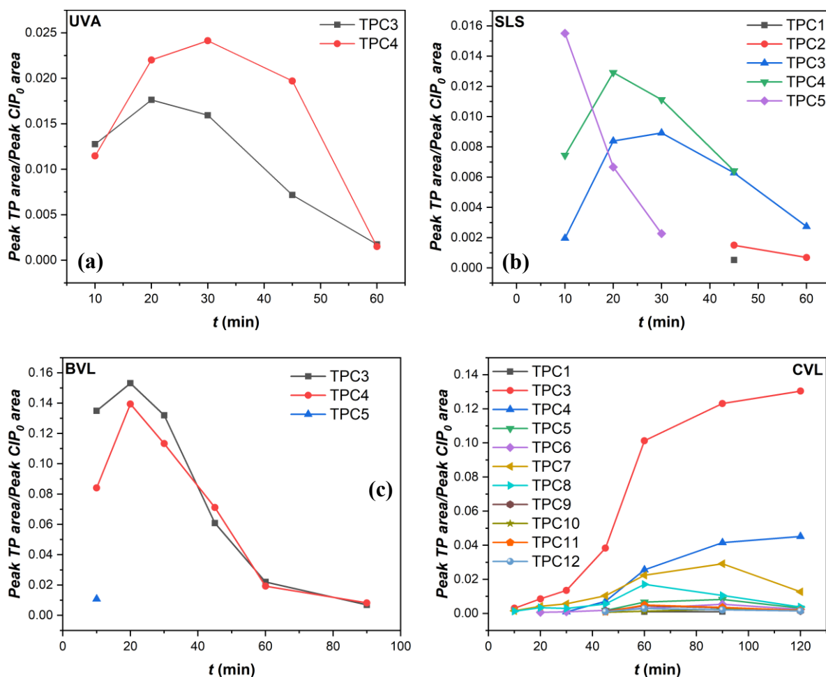
Figure 58. Transformation byproducts profile generated during the photocatalytic degradation of ciprofloxacin (CIP) by N/TiO 2 /rGO@Al 2 O 3 foam under UVA light (a), solar light simulator (SLS)(b), blue visible light (BVL)(c) and cold visible light (CVL) (d).
