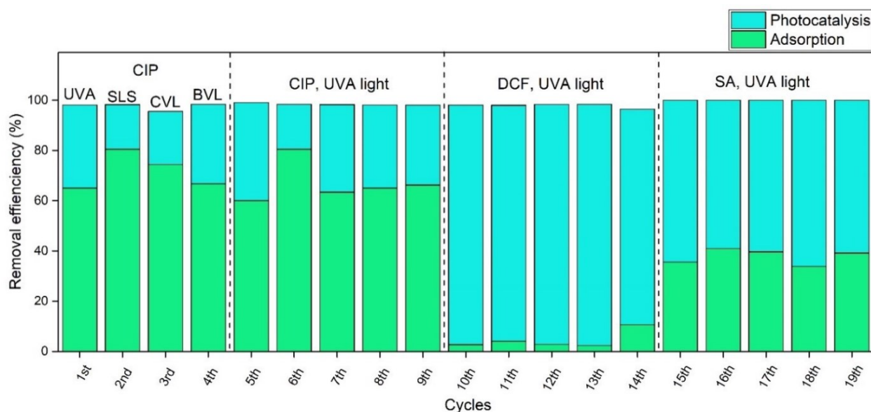
Figure 57. Reusability and stability tests for 19th consecutive cycles. Photocatalytic degradation of ciprofloxacin (CIP) by N/TiO 2 /rGO@Al 2 O 3 foam under UVA light, Solar light simulator (SLS), cold visible light (CVL) and blue visible light (BVL). Photocatalytic degradation of ciprofloxacin (CIP), diclofenac (DCF), and salicylic acid (SA) by N/TiO 2 /rGO@Al 2 O 3 foam under UVA light.
