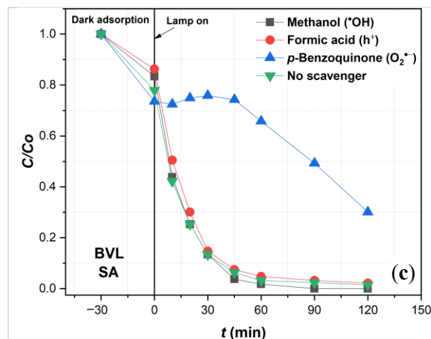
Figure 47. Photocatalytic salicylic acid (SA) degradation by N/TiO 2 /rGO with 0.25 wt. % of rGO material in the presence of different scavenger agents under (a) UVA light, (b) solar light simulator (SLS), and (c) blue visible light (BVL). Tests with scavengers were not carried out under CVL for SA due to the minimal photoactivity observed under this irradiation source.
