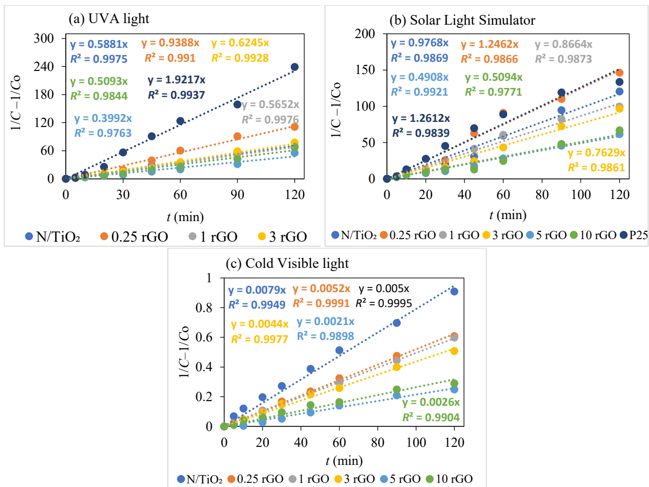
Figure S8. Pseudo-second order kinetic rate of the photocatalytic degradation of ciprofloxacin by Degussa P25 N/TiO 2 and N/TiO 2 /rGO samples under (a) UVA light (lamp I), (b) solar light simulator lamp (II), and (c) Cold visible light (lamp III).
