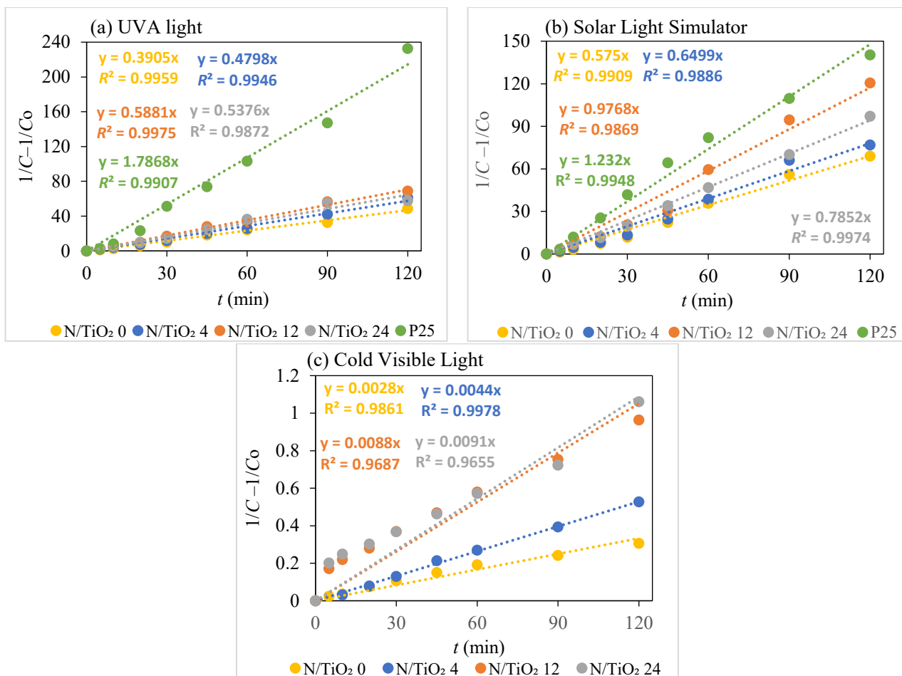
Figure S6. Pseudo-second order kinetic rate of the photocatalytic degradation of ciprofloxacin by Degussa P25 TiO 2 and N/TiO 2 samples under (a) UVA light (lamp I), (b) solar light simulator lamp (II), and (c) Cold visible light (lamp III).
